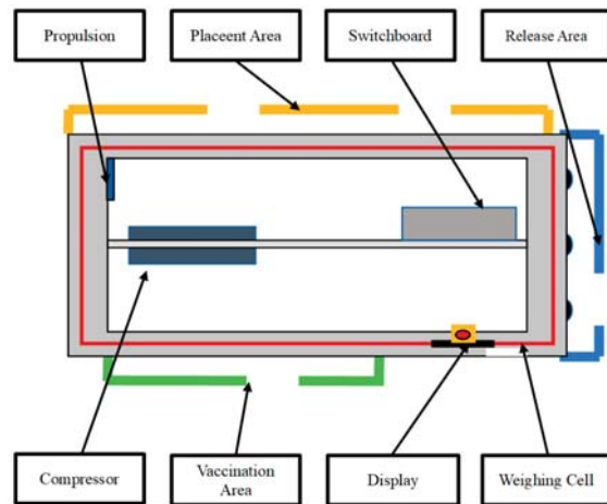
Image 2 - Schematic representation (Plan view) of grading device
